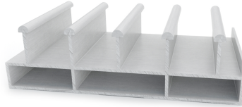
RİO BST 605 Eşikli Alt Ray Lower Rail (Threshold) (1,14 kg/mt)
